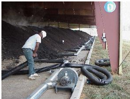
Figure A-14-3. Forced aeration systems, or aerated static piles, use blowers to provide oxygen into the compost pile instead of turning or moving the pile. Photo: Jason Governo, U. of Georgia
