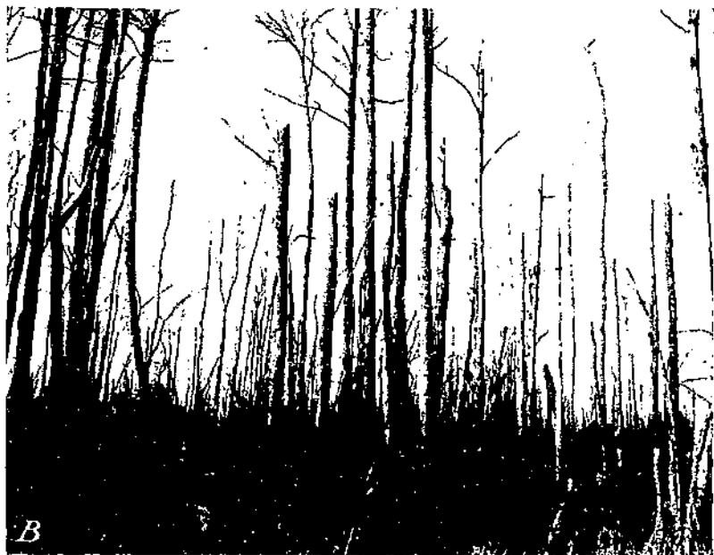
A, Pond formed as a result of accelerated sedimentation at boring range EG-4, East Goose Valley; B, trees in Goose Valley, between boring ranges G-7 and G-8, killed by the high water table caused by filling of the Wells drainage ditch.
