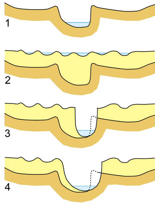
Fig. 3. Four phases of an aggradation-degradation episode (ADE): (1) single thread channel prior to disturbance; (2) channel and floodplain aggrade; possibly forming a braided channel, in response to sediment loads in excess of transport capacity; (3) as sediment loads return to background levels, channels rejoin and incise down to original levels; (4) channels widen over a longer period of time. See James and Lecce (2013) for description of ADEs.
