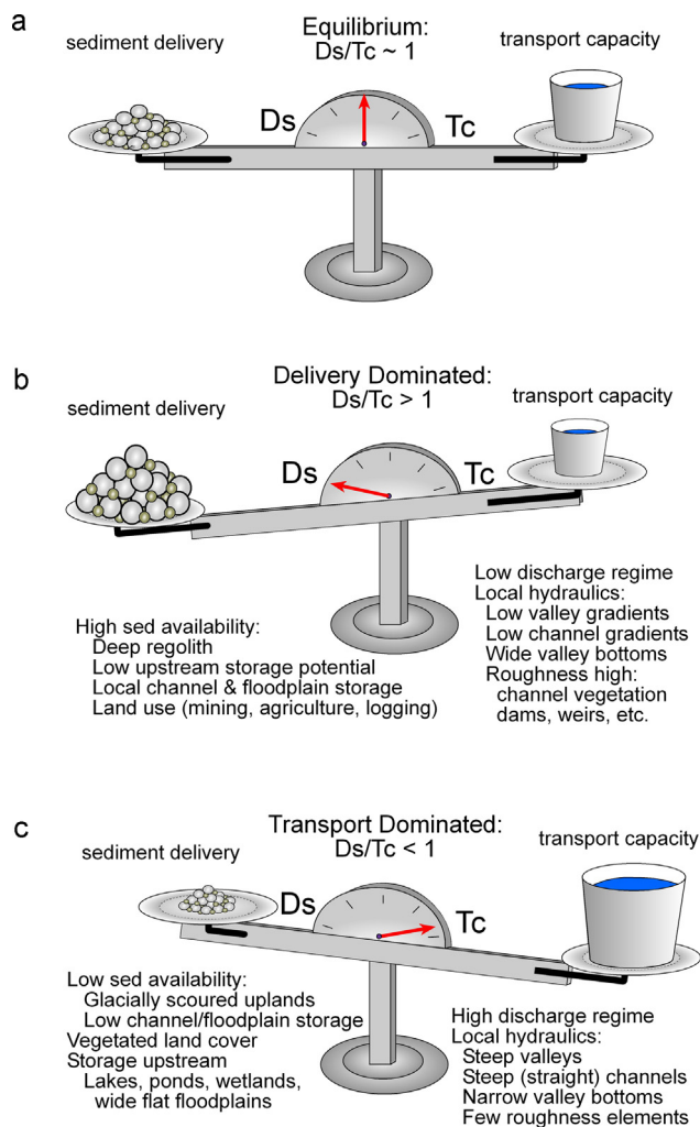
Fig. 7. Triple-beam balance metaphor for sediment storage potential: (A) sediment delivery ( D_s ) equals transport capacity ( T_c ) so channel is in equilibrium; i.e., no change in storage; (B) D_s > T_c so net gain of sediment, aggradation, and high LS storage potential; (C) D_s < T_c so net loss of sediment, degradation, and LS recruited from reach.
